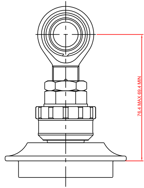
ADJUSTABLE END OPTION
