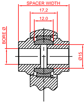
BEARING END DETAIL
